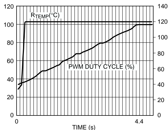
Figure 78. Enhanced Acoustics Mode with Ramp Rate = 8
