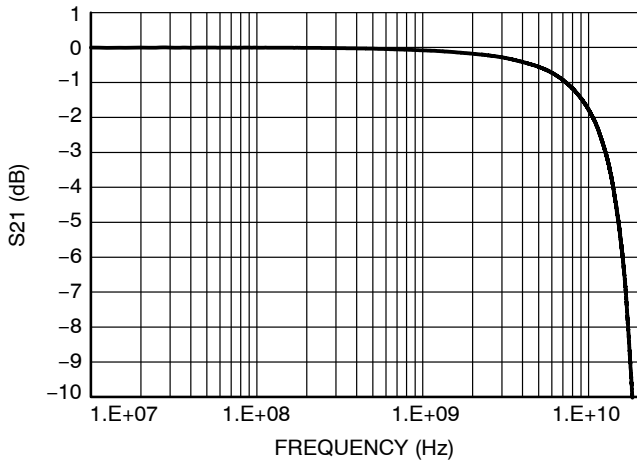
Figure 5. Insertion Loss
