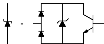
Figure 1. Pin Schematic
