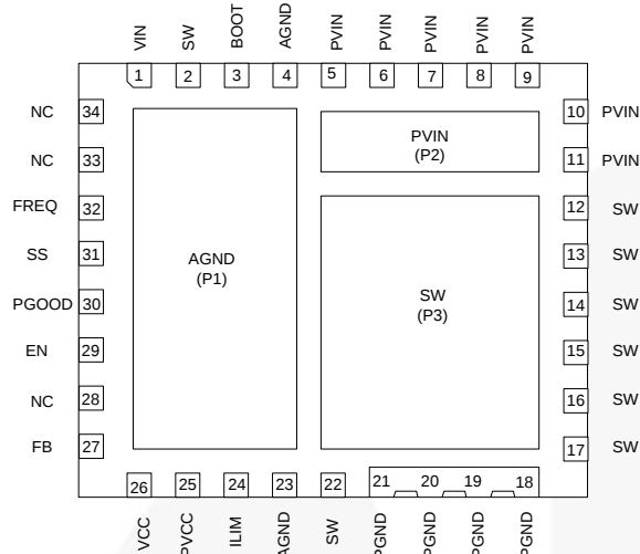
Figure 4. Pin Assignments(Bottom View)
