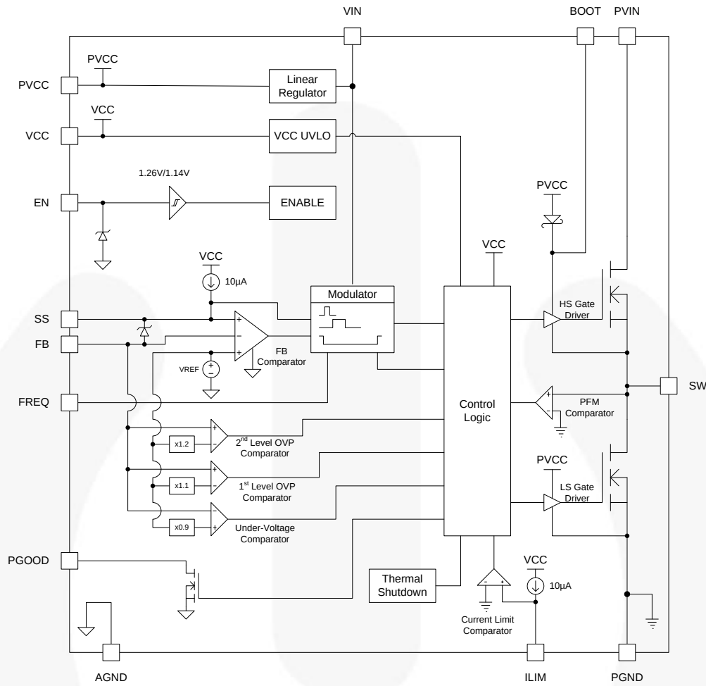
Figure 3. Block Diagram
