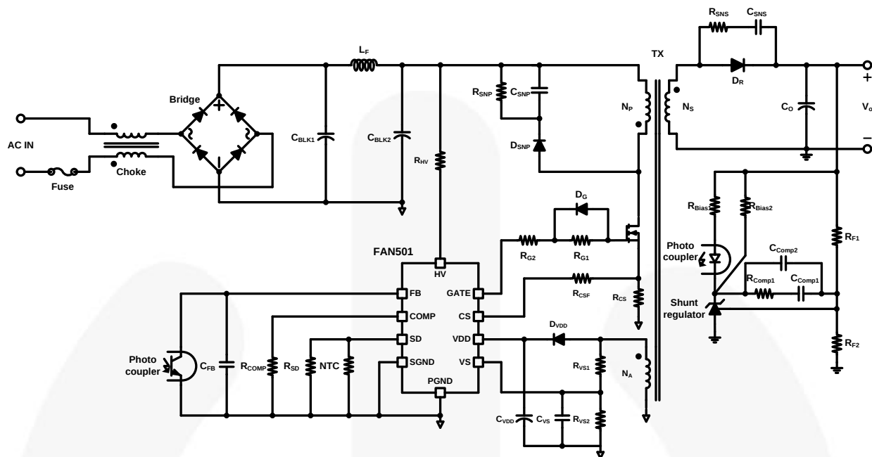
Figure 2. Typical Application
