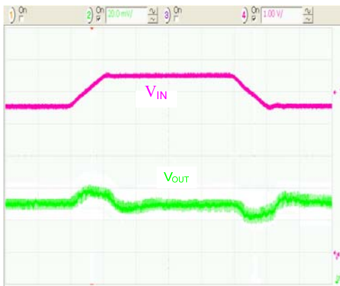
Figure 21. Line Transient Response in PWM Mode, 10\text{ }\mu\text{s/div} .
