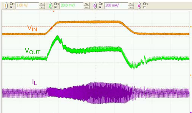
Figure 19. Line Transient at V_{IN} = 3.2\text{ V} to 4.2\text{ V} , 300 mA Load, t_{RISE} = t_{FALL} = 10\text{ }\mu\text{s} , 20 \mu\text{s} /div.
