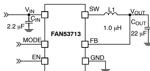
Figure 1. Typical Application
