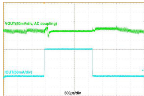
Figure 15. Load Transient, V_{IN} = 3.6\text{ V} , V_{OUT} = 1.8\text{ V} , 10\text{ mA} \leftrightarrow 150\text{ mA} , 1\text{ μs} Edge, Auto Mode
