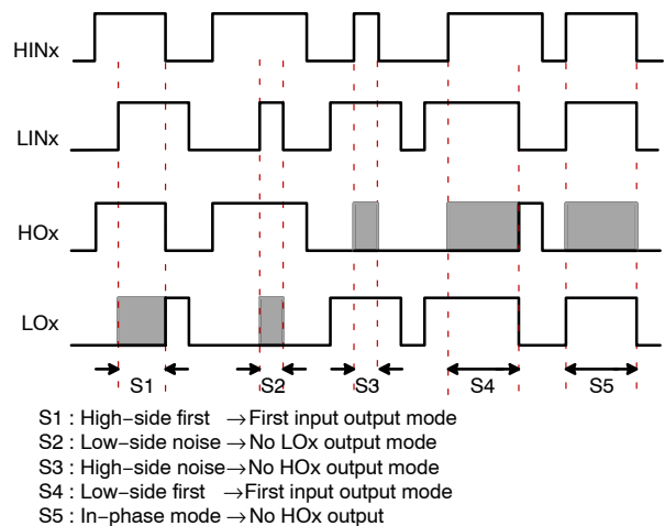
Figure 40. Interlock Function
