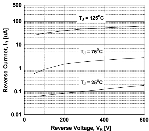
Figure 20. Reverse Current
