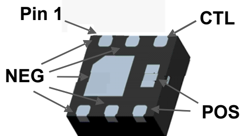
Figure 3. Pin Assignments
