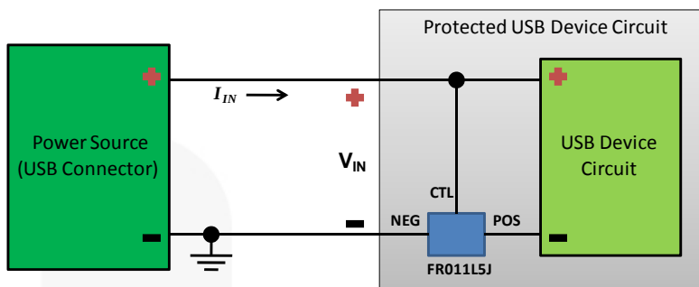
Figure 2. Typical Schematic
