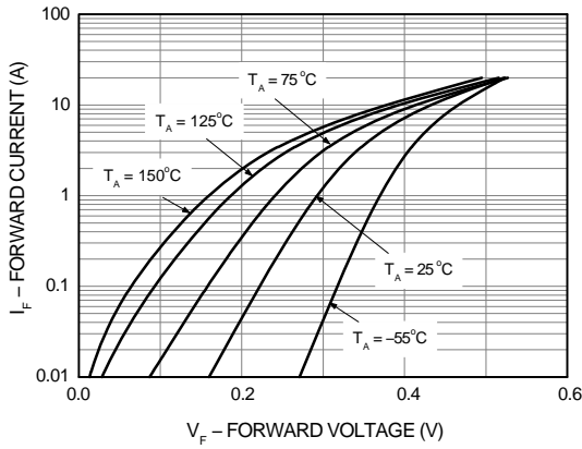
Figure 3. Typical Forward Characteristics
