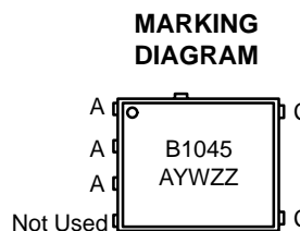
SO-8 FLAT LEAD CASE 488AA STYLE 2
