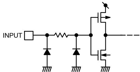
Figure 5. Input Equivalent Circuit
