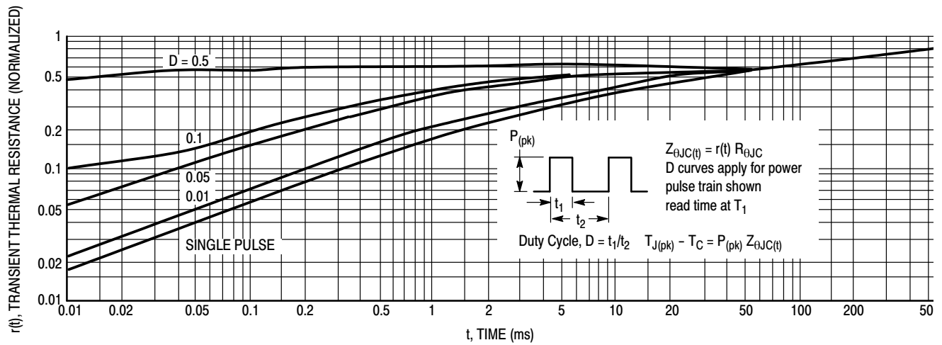
Figure 5. Thermal Response
