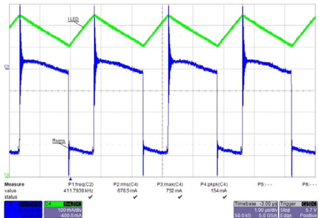
Figure 33. Voltage Measured on R_{CS} (R4)
