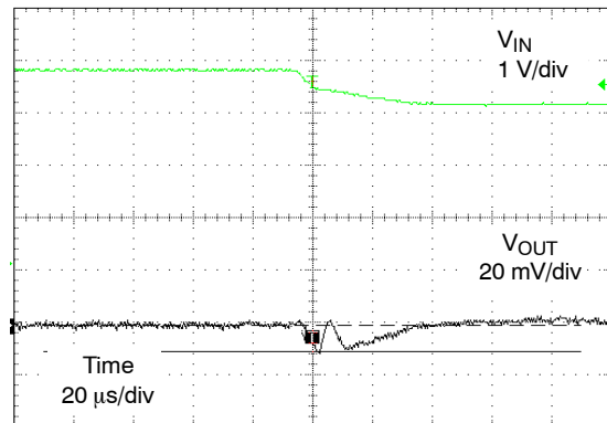
Figure 18. 3.6 V to 3.0 V Line Transient (\text{Risettime} = 50 \mu\text{s}, V_{OUT} = 1.2 \text{ V}, I_{OUT} = 100 \text{ mA}, T_A = 25^\circ\text{C})
