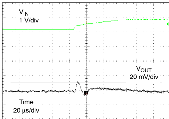
Figure 17. 3.0 V to 3.6 V Line Transient (\text{Risettime} = 50 \mu\text{s}, V_{OUT} = 1.2 \text{ V}, I_{OUT} = 100 \text{ mA}, T_A = 25^\circ\text{C})
