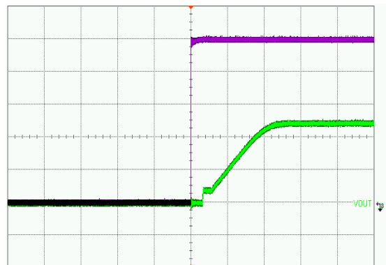
( V_{IN} = 5\text{ V} , I_{LOAD} = 10\text{ mA} , L = 3.3\text{ }\mu\text{H} , C_{OUT} = 20\text{ }\mu\text{F} \times 2 ) Upper Trace: Input Voltage, 1 V/div Lower Trace: Output Voltage, 500 mV/div Time Base: 500 \mu\text{s} /div
