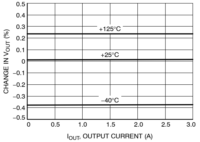
Figure 7. Load Regulation
