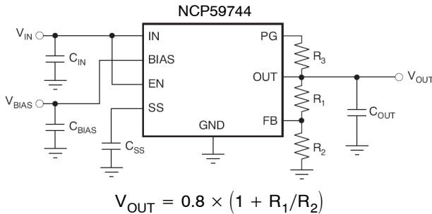
Figure 25. Typical Application Schematics
