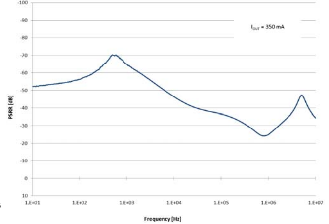
Figure 13. V_{IN} Power Supply Ripple Rejection vs. Frequency
