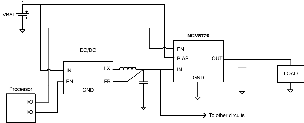
Figure 3. Typical Application: Low-Voltage Post-Regulator with ON/OFF functionality
