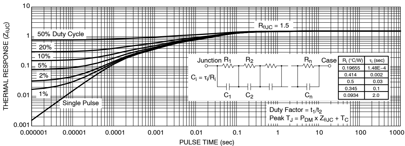
Figure 21. Diode Transient Thermal Impedance
