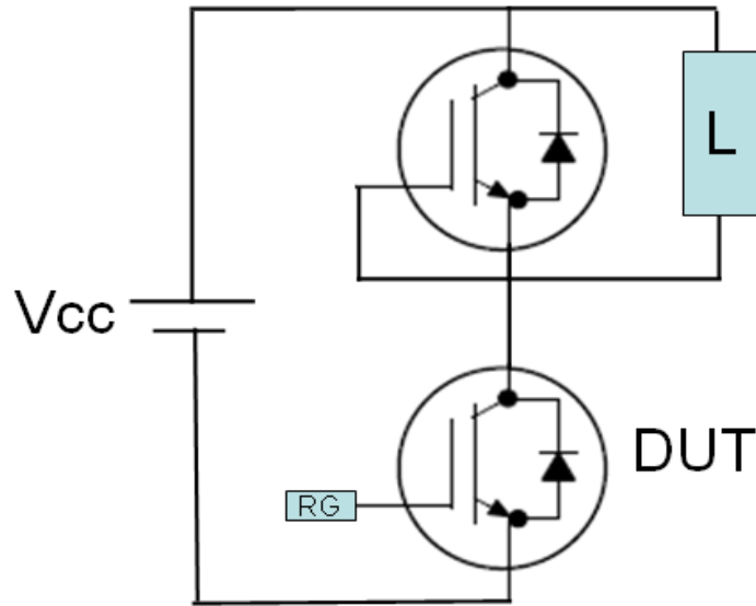
Figure 19. Test Circuit for Switching Characteristics
