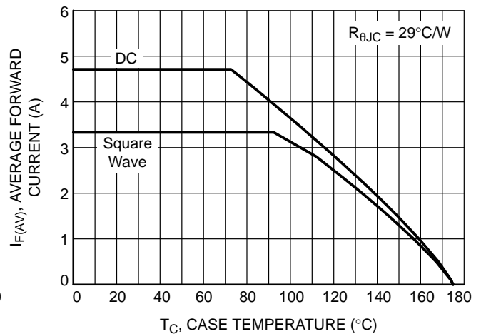
Figure 6. Current Derating
