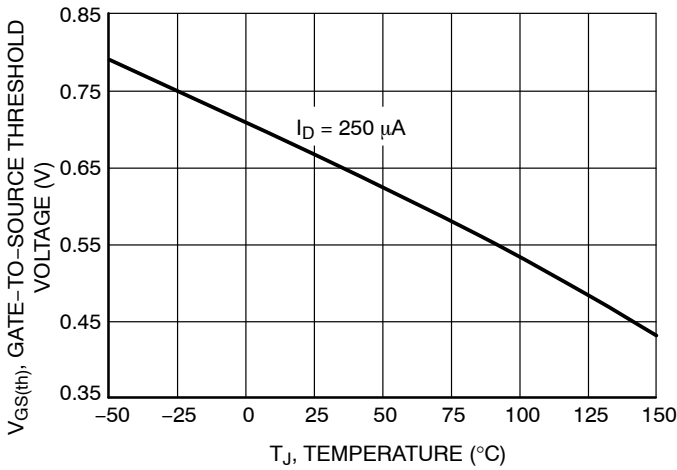
Figure 17. Threshold Voltage
