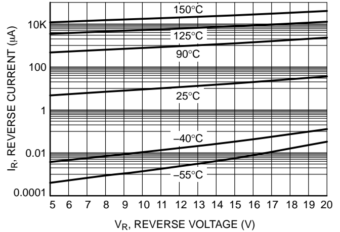
Figure 6. Leakage Current
