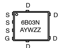
DFN5 (SO-8FL) CASE 506EZ
