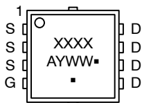
WDFN8 CASE 511AB WDFNW8 CASE 515AN
