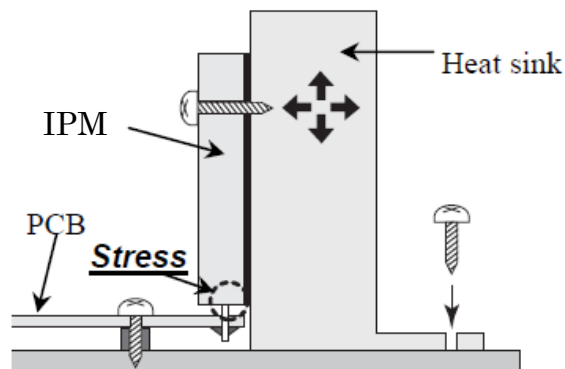
Figure 22. Fix to Heat Sink
