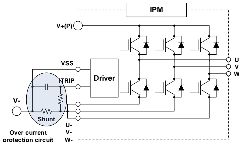
Figure 9. Over-current protection circuit setting
