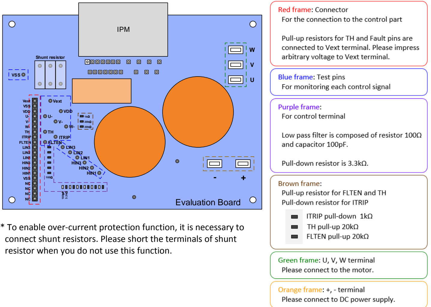
Figure 26. Description of each pin
