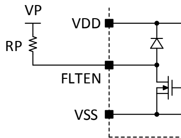
Figure 21. Fault Connection
