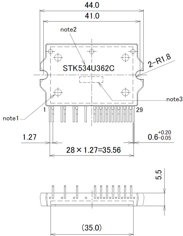
Figure 23. Package Outline
