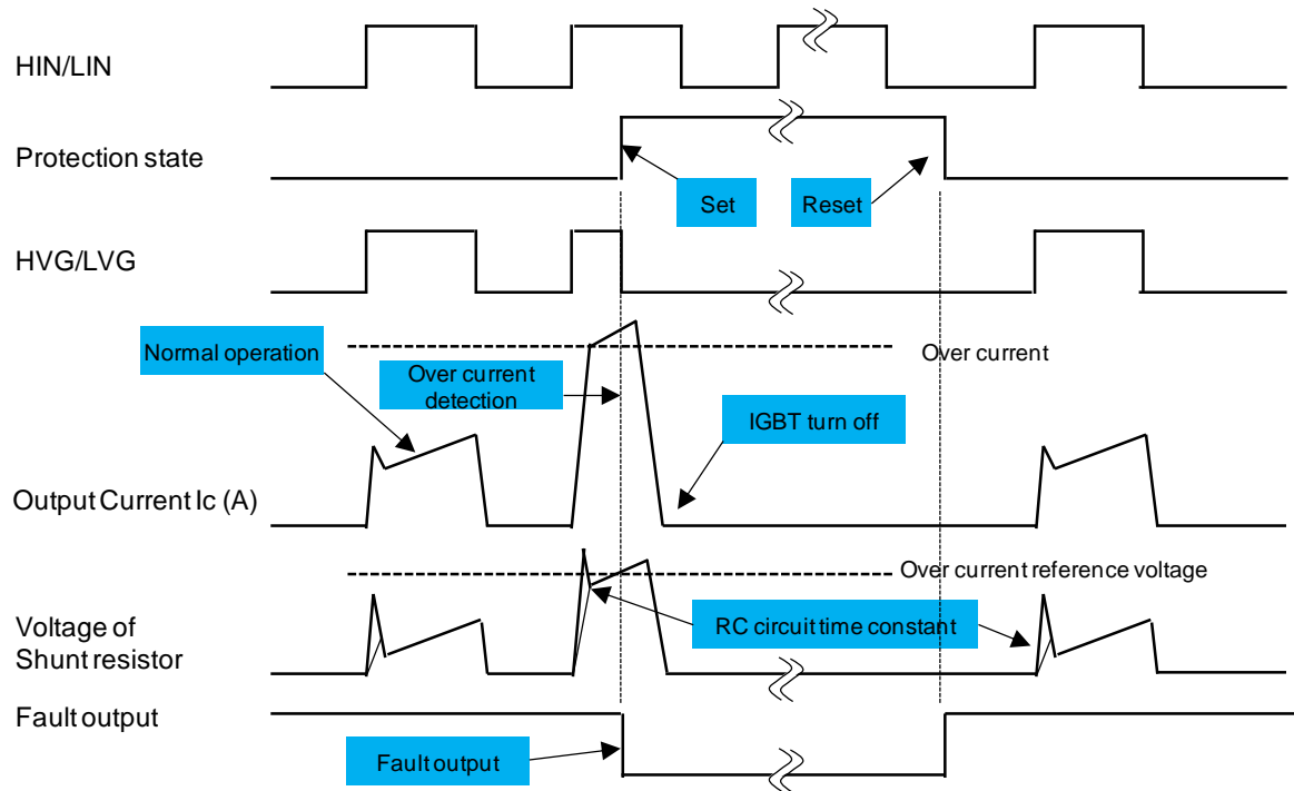
Figure 11. Over current protection Timing chart
