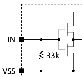
Figure 20. Internal Input Circuit
