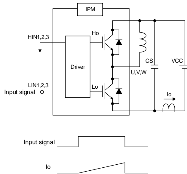
Figure 6. R.B.SOA circuit
