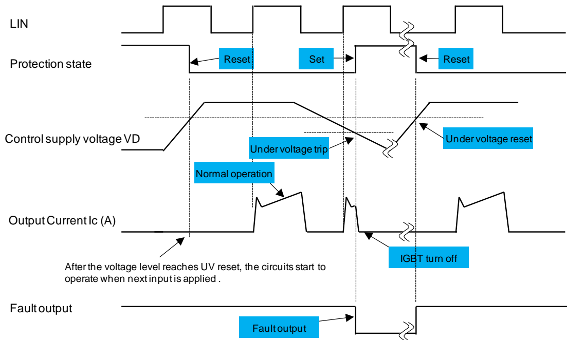
Figure 12. Low side UVLO timing chart
