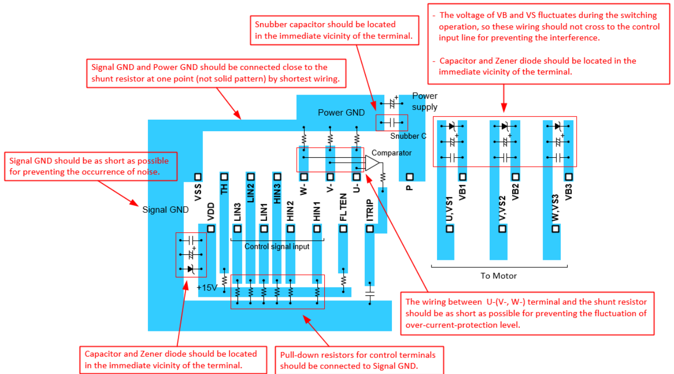
Figure 18. PCB design reference
