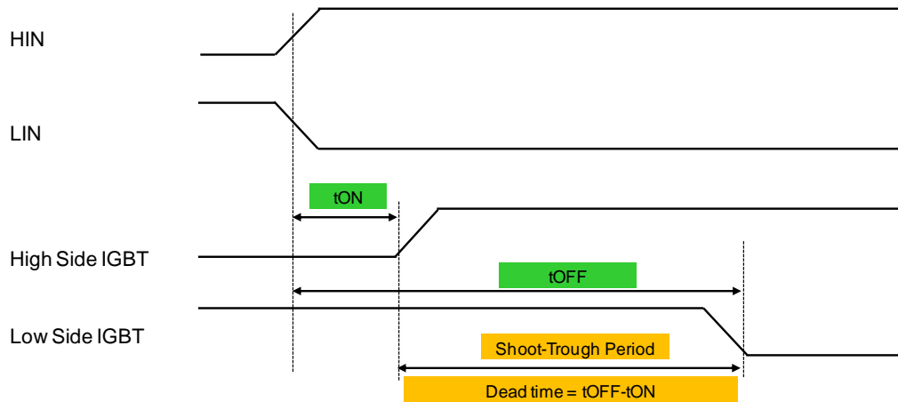
Figure 16. Shoot Trough Period
