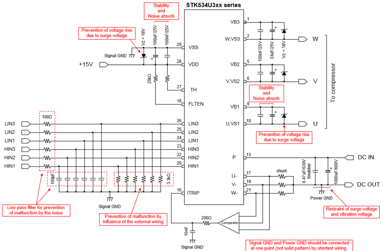
Figure 17. STK534U3xx series application circuit
