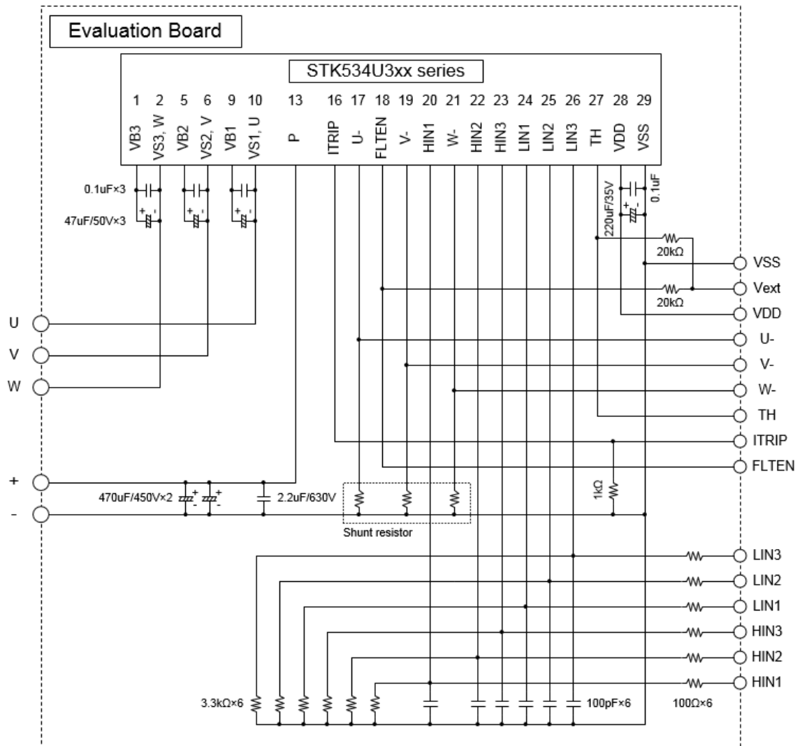
Figure 24. Evaluation board schematic
