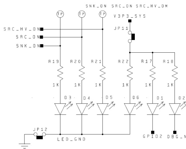
Figure 5. LED Indicators
