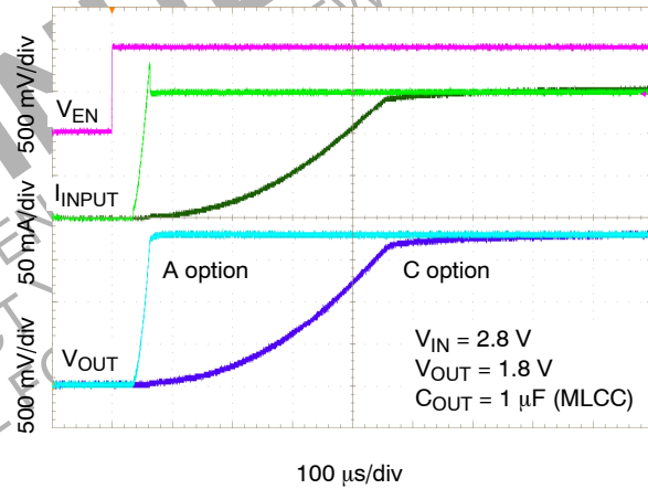
Figure 31. V_{OUT} Slew-Rate Comparison A and C option - I_{OUT} = 150 \text{ mA}
