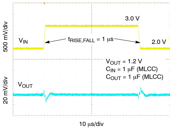
Figure 33. Line Transient Response - I_{OUT} = 150 \text{ mA}
