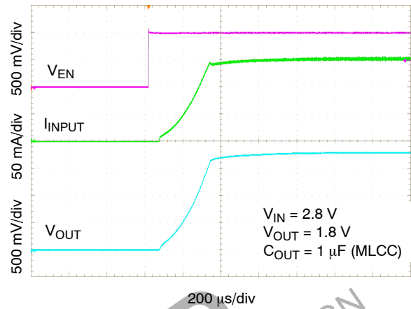
Figure 29. Enable Turn-on Response - I_{OUT} = 150 \text{ mA} , Slow Option - C
