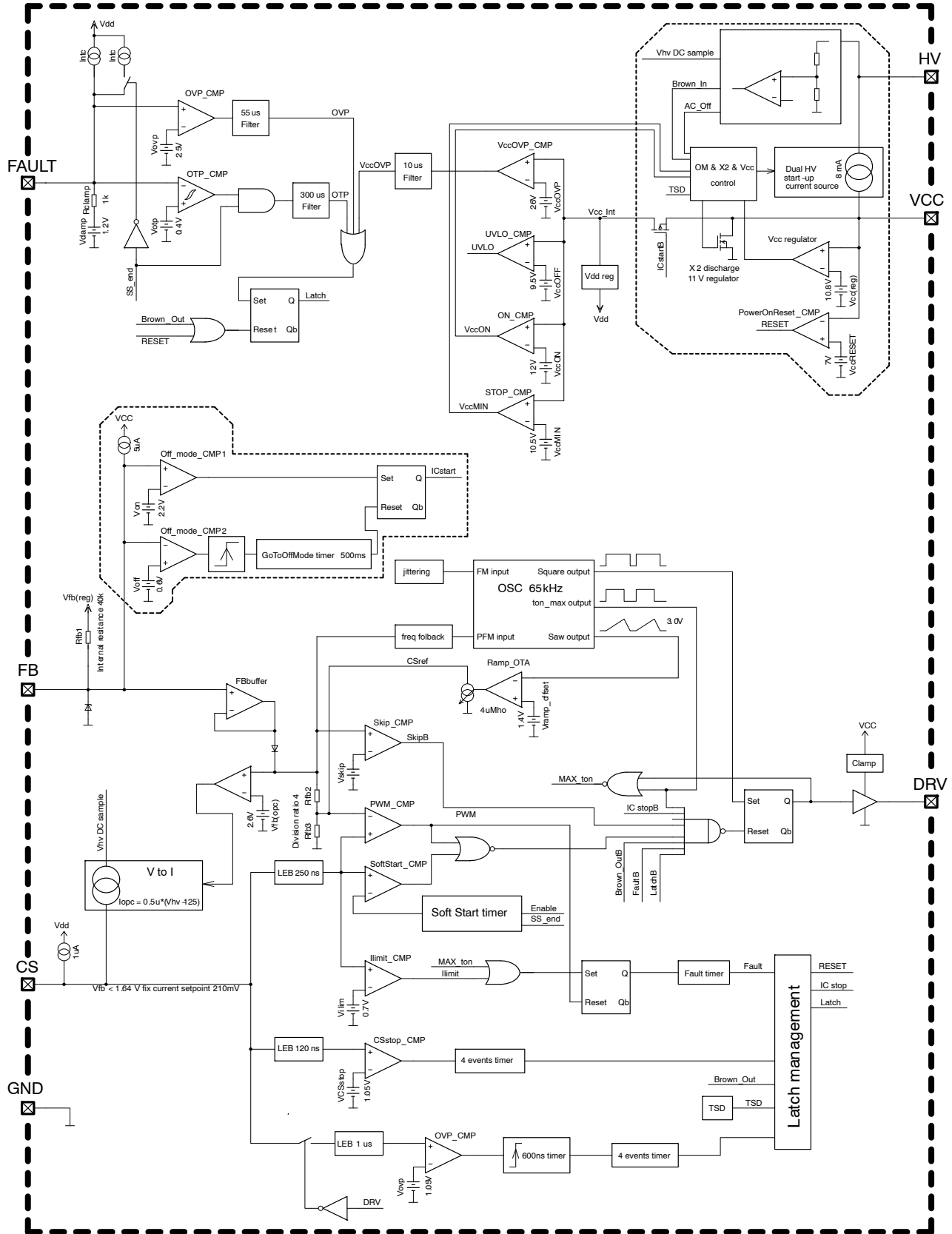
Figure 2. Simplified Internal Block Schematic
