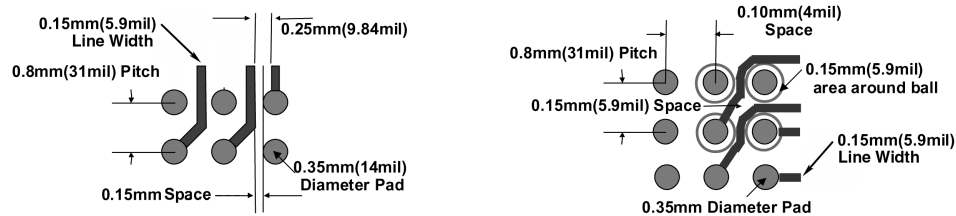
FIGURE 2. BGA Routing
