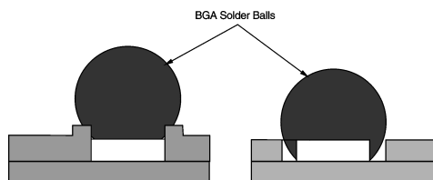
FIGURE 15. Cross-section Comparison of Solder Mask Defined Pad (left) to Non-Solder Mask Defined Pad (right) with BGA Solder Ball Connections
