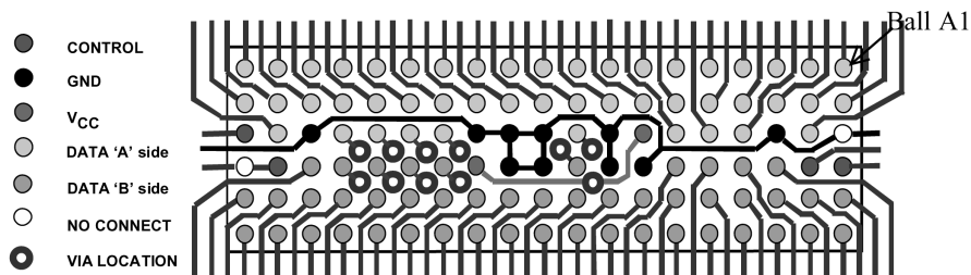
FIGURE 10. 114-Ball 48-Bit BGA with Vias (FST32211)
