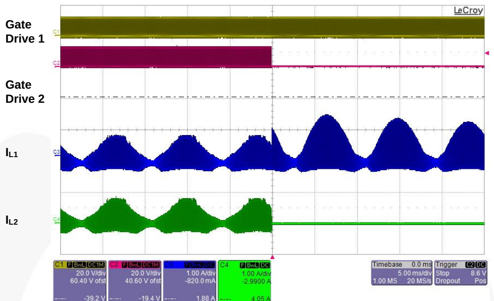
Figure 31. Phase-Shedding Operation
