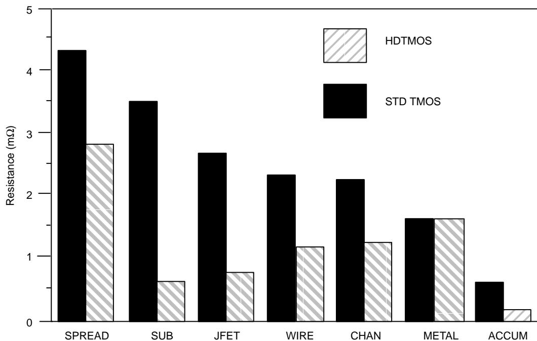
Figure 3. On-Resistance Components
