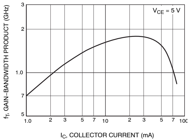
Figure 4. f_T - I_C
