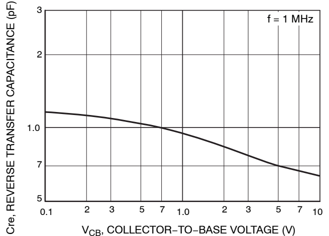
Figure 6. C_{re} - V_{CB}
