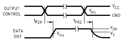
FIGURE 2. Waveforms (Input Pulse Characteristics; f=1MHz , t_r=t_f=3ns )
