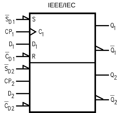
Figure 3. Logic Symbols
