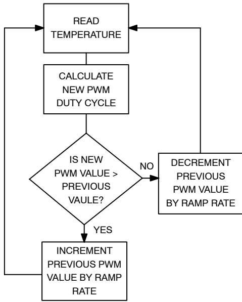
Figure 28. Filtered Mode Algorithm
