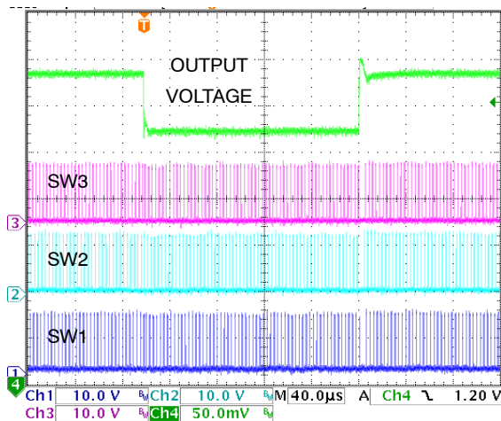
Figure 10. Load Transient
