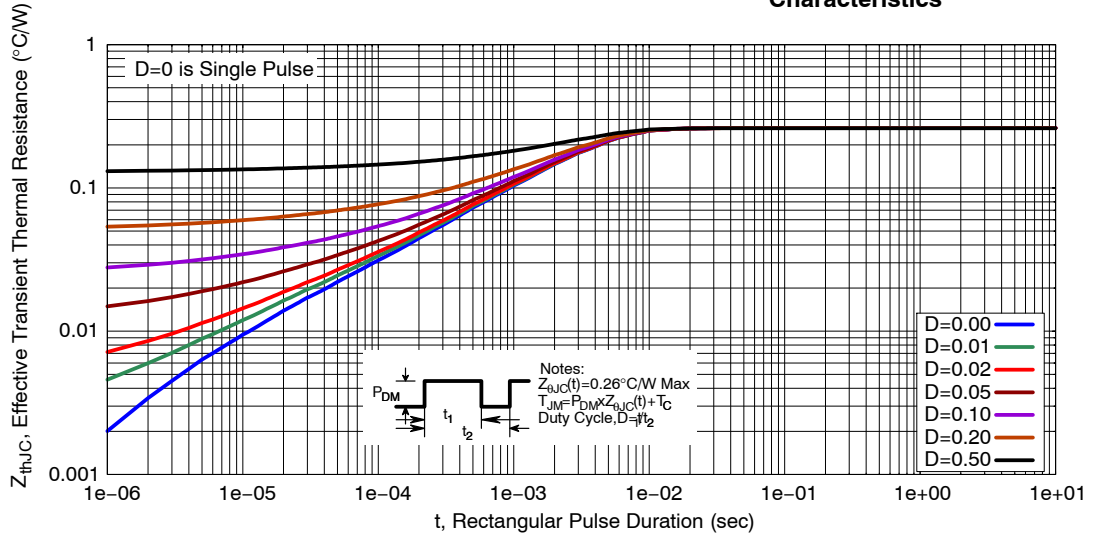
Figure 21. Transient Thermal Impedance of IGBT
