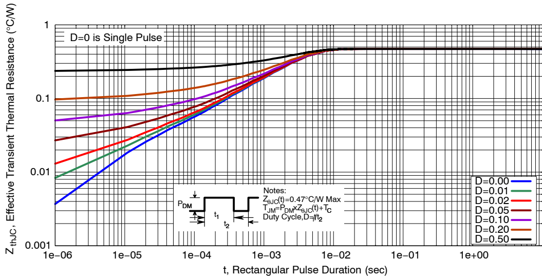
Figure 22. Transient Thermal Impedance of Diode
