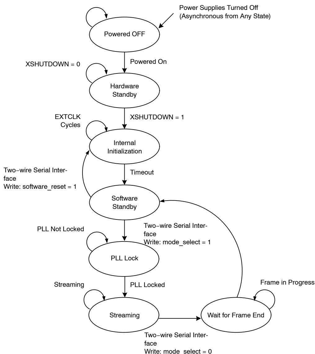
Figure 5. System States
