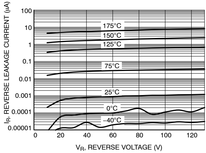
Figure 5. Reverse Current – BASH19
