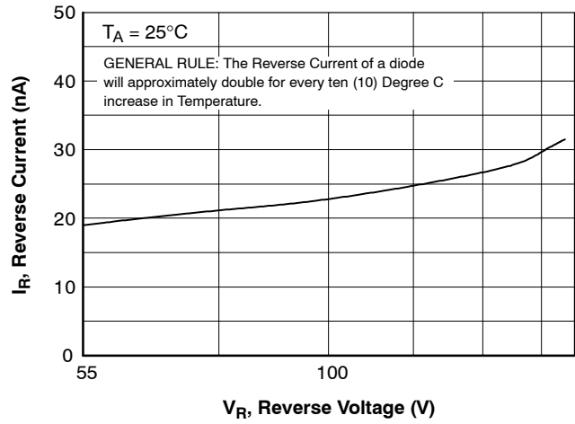
Figure 2. Reverse Current vs. Reverse Voltage I_R - 55 \text{ to } 205 \text{ V}
