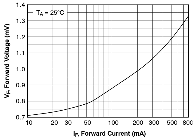
Figure 6. Forward Voltage vs. Forward Current V_F - 10 \text{ to } 800 \text{ mA}
