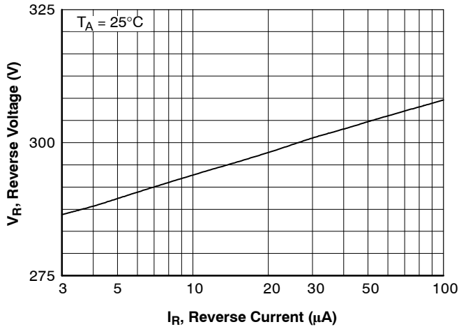
Figure 1. Reverse Voltage vs. Reverse Current B_V - 1.0 \text{ to } 100 \mu\text{A} T_A = 25^\circ\text{C}
