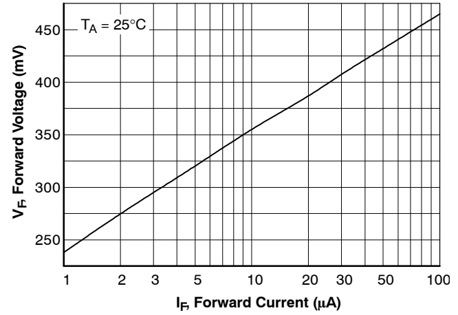
Figure 4. Forward Voltage vs. Forward Current V_F - 1.0 \text{ to } 100 \mu\text{A}
