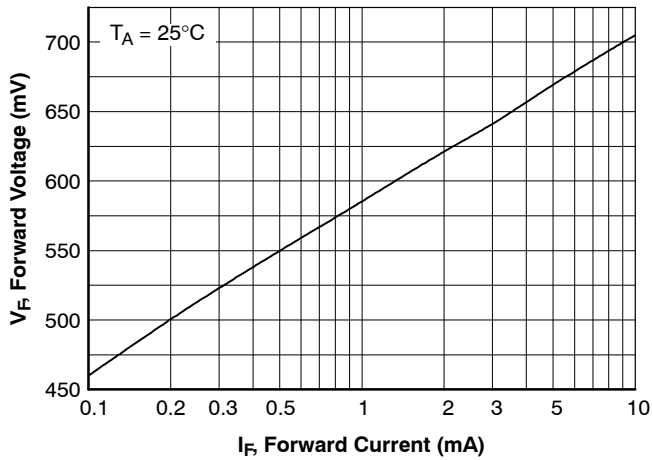
Figure 5. Forward Voltage vs. Forward Current V_F - 0.1 \text{ to } 10 \text{ mA}
