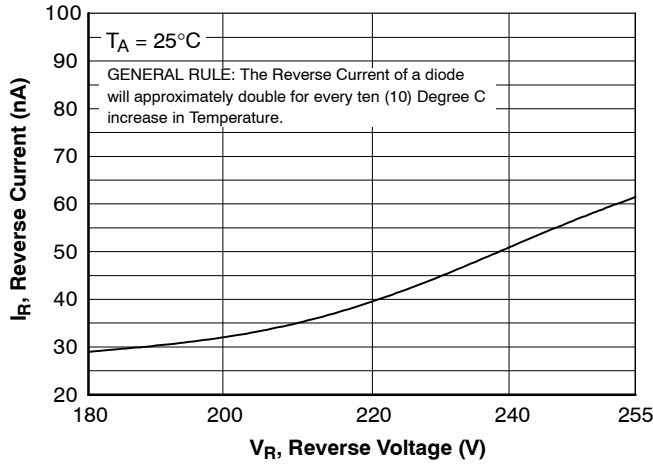
Figure 3. Reverse Current vs. Reverse Voltage I_R - 180 \text{ to } 225 \text{ V}
