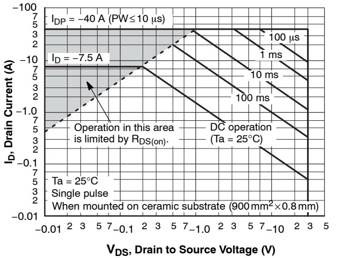
Figure 11. SOA
