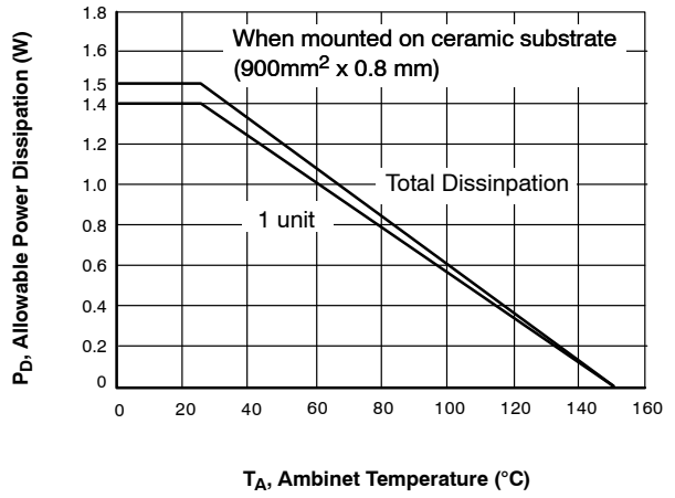
Figure 12. P_D - T_A
