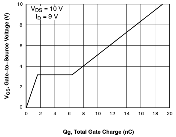
Figure 10. V_{GS} - Q_g
