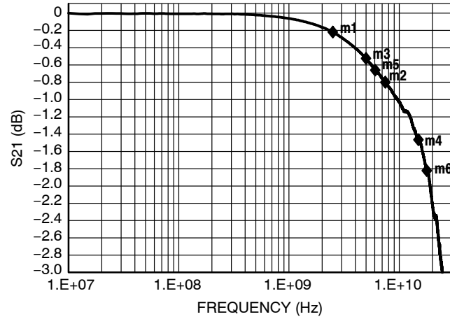
Figure 9. Insertion Loss
