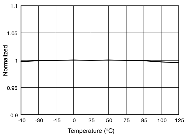
Figure 11. Reference Voltage of Constant Current ( V_{VR-CC} ) vs. Temperature
