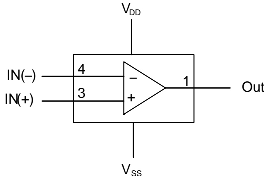
Figure 1. Functional Diagram
