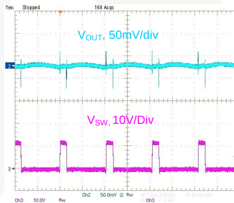
Figure 27. V_{OUT} Ripple and SW Voltage, 10 A Load
