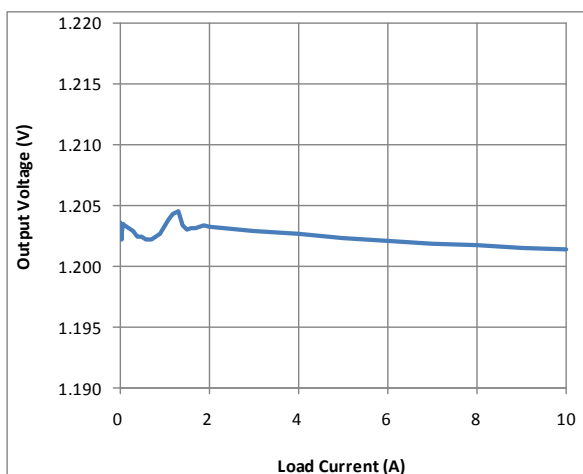
Figure 9. Load Regulation
