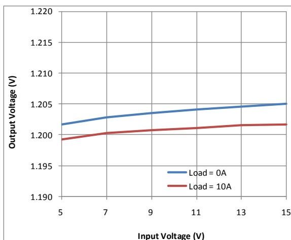
Figure 10. Line Regulation
