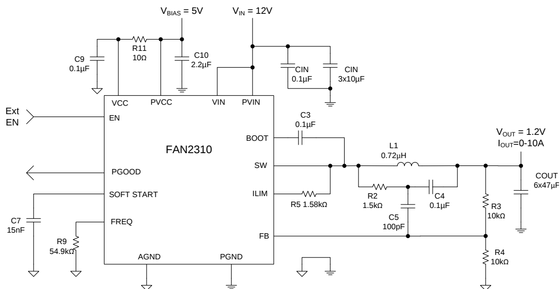
Figure 1. Typical Application
